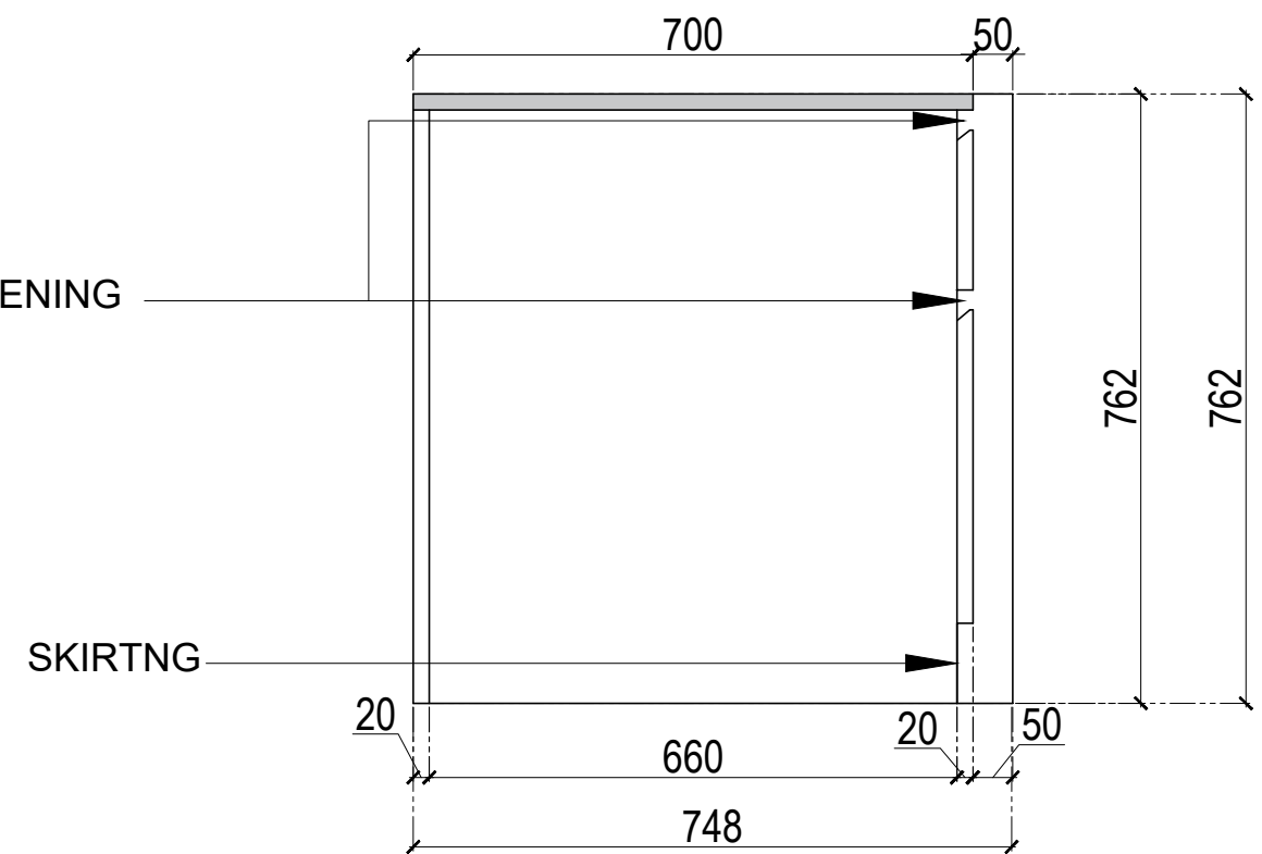
3 SIDE ELEVATION WORK STATION
