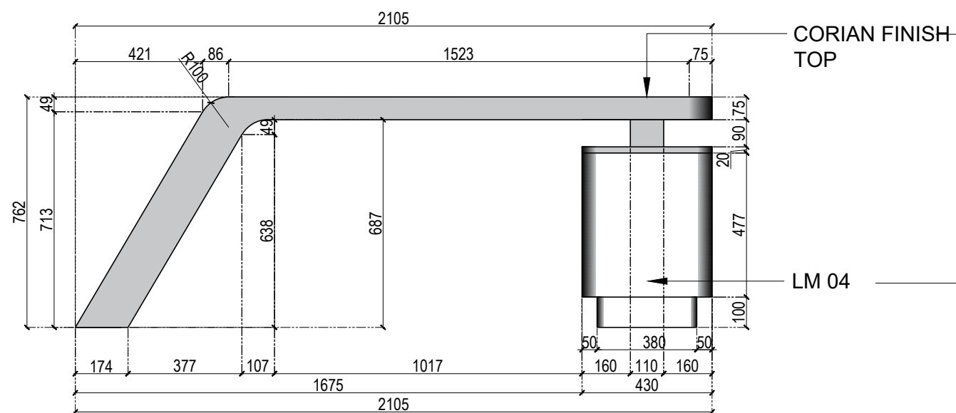
2 ELEVATION AT A DIRECTOR ROOM
