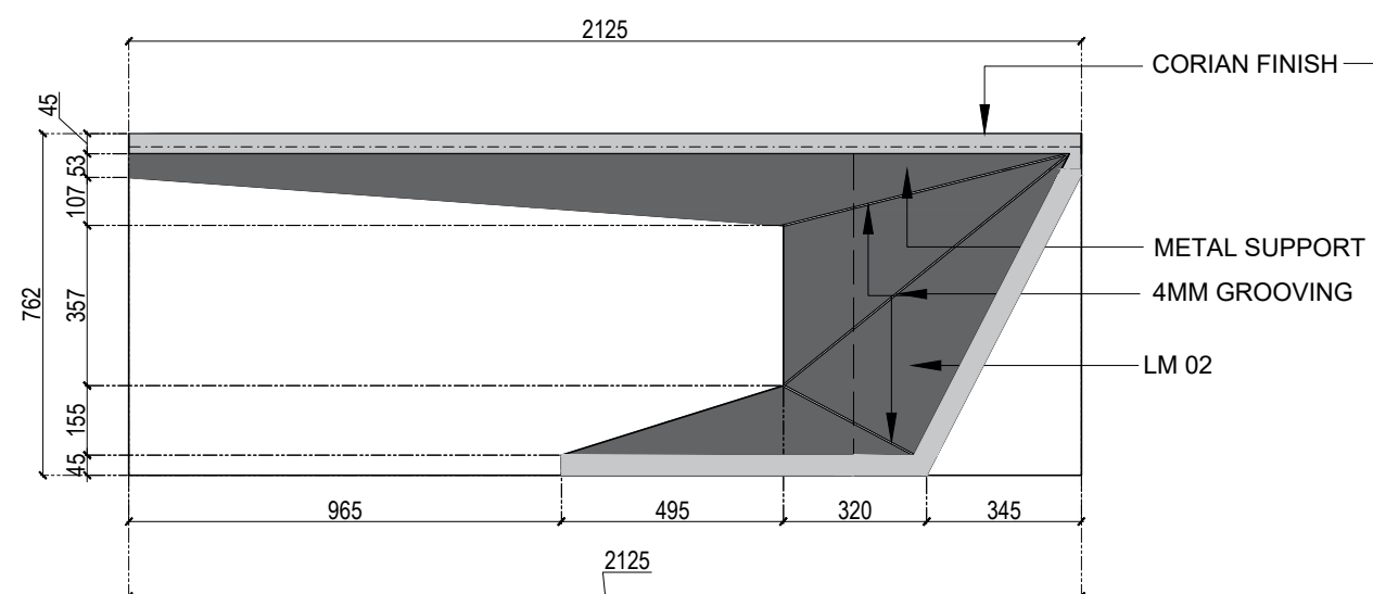
2 ELEVATION AT A MD WORKING TABLE
