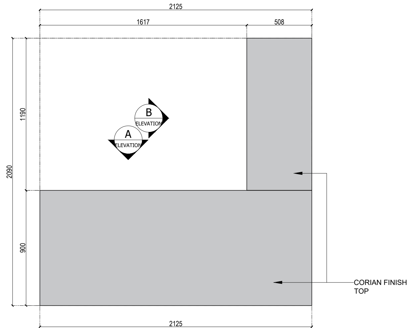
1 PLAN MD WORKING TABLE
