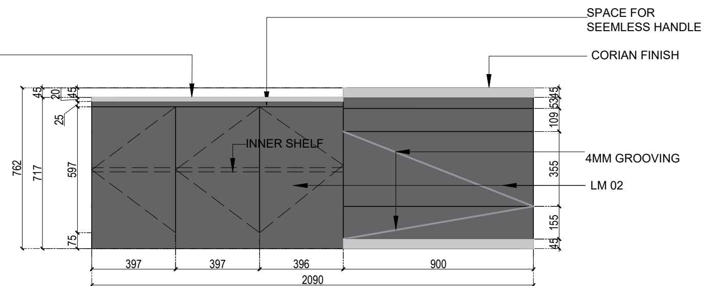
3 ELEVATION AT B MD WORKING TABLE
