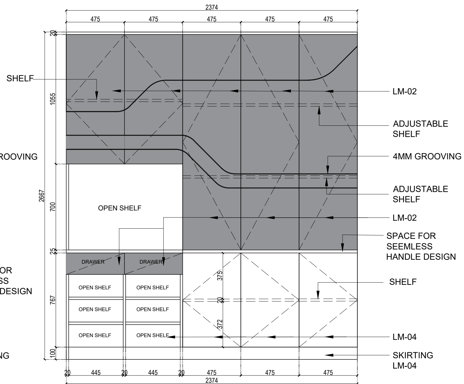
2.1 FRONT ELEVATION WORKSTATION AREA
