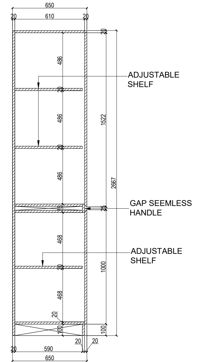
3 SECTION DB CABINET
