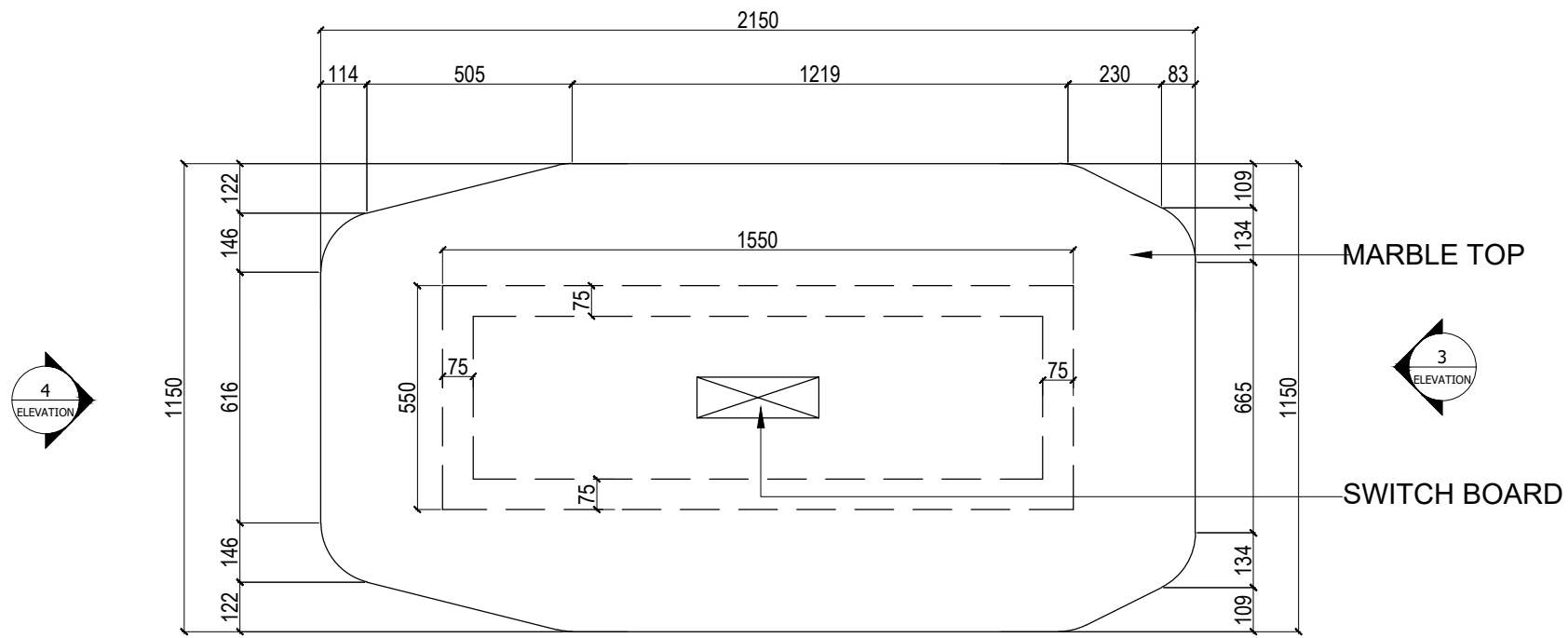
1 PLAN MEETING TABLE
