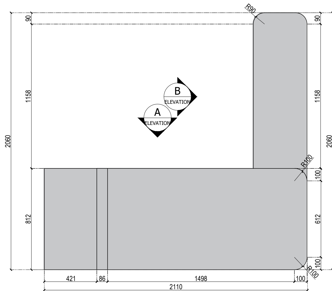
1 PLAN DIRECTOR ROOM
