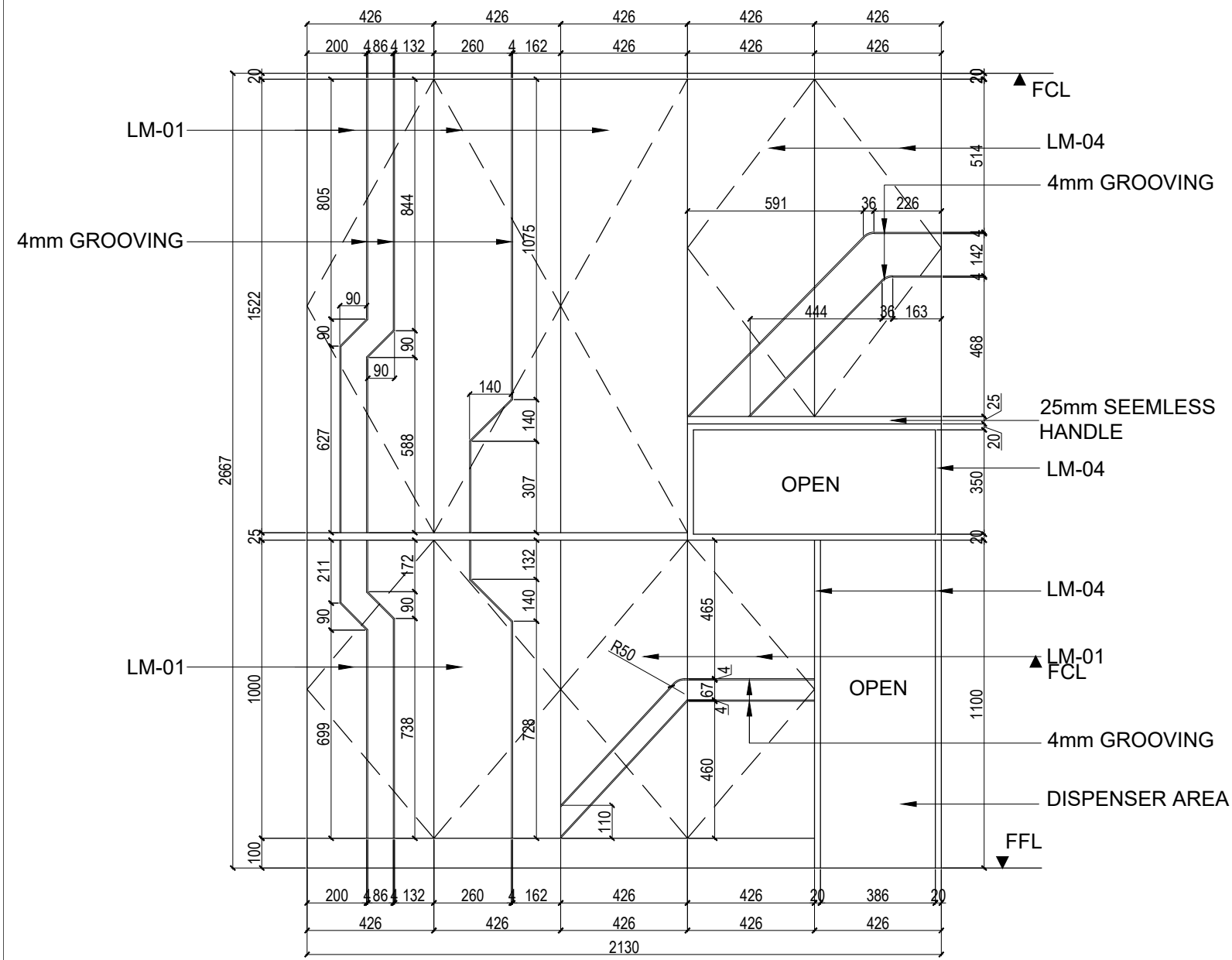
2 FRONT ELEVATION DB CABINET
