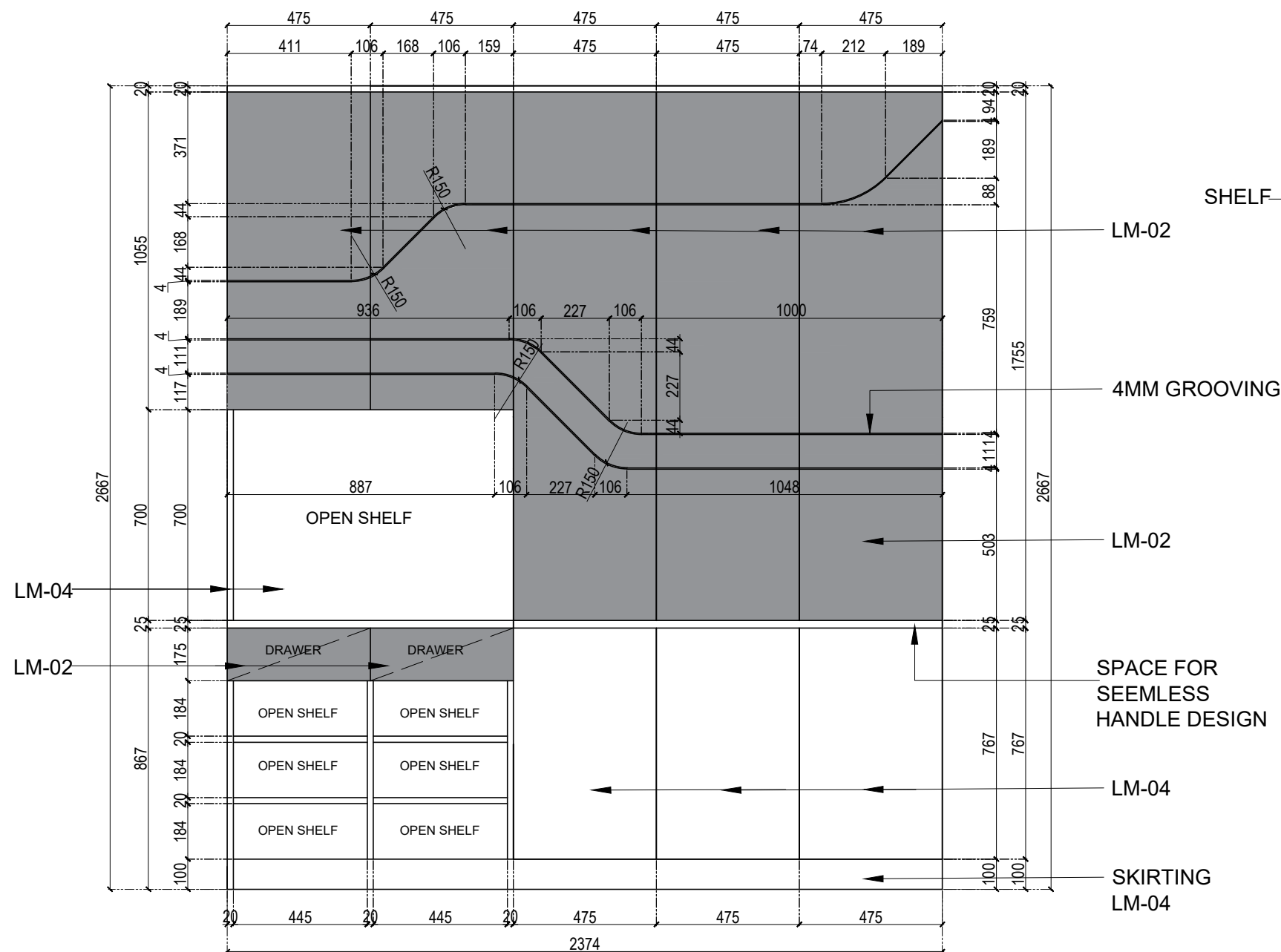
2 FRONT ELEVATION WORKSTATION AREA
