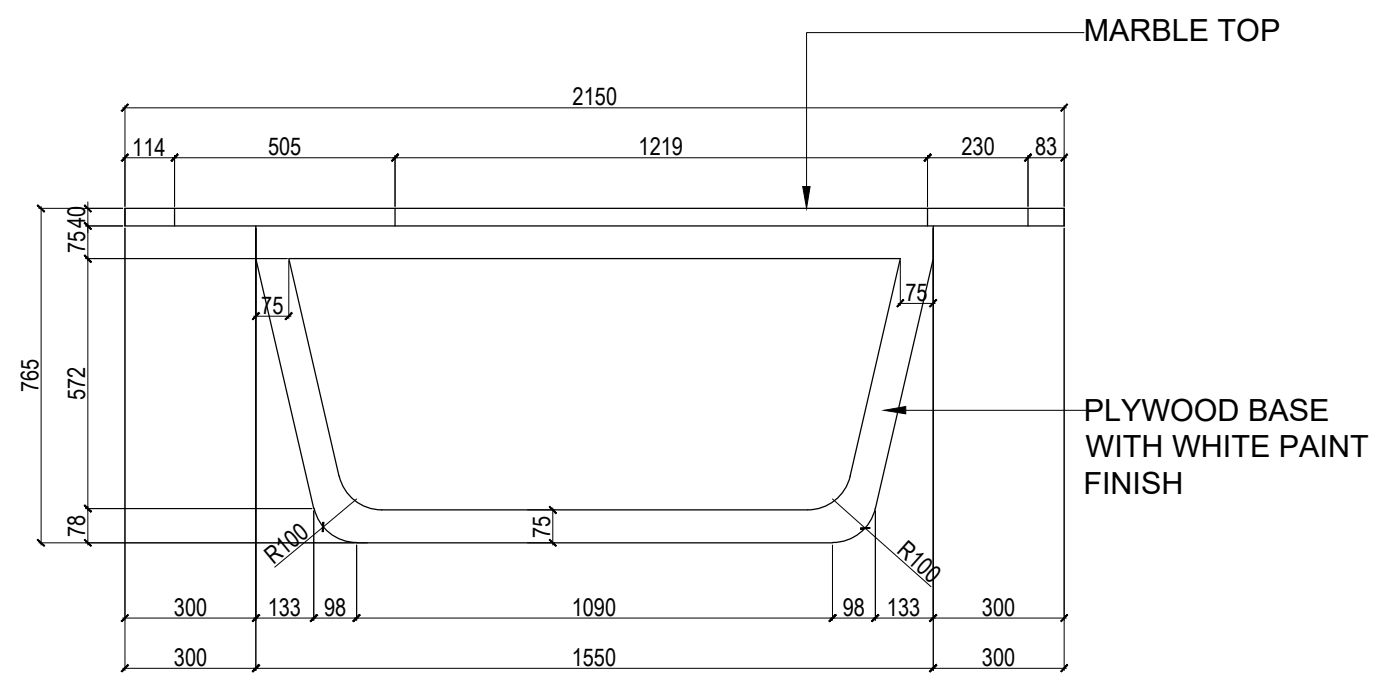
2 ELEVATION MEETING TABLE
