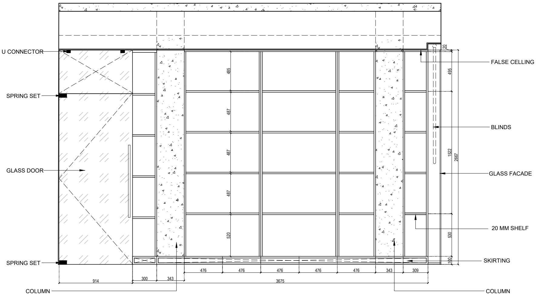
4 INNER ELEVATION MD STORAGE CABINETE
