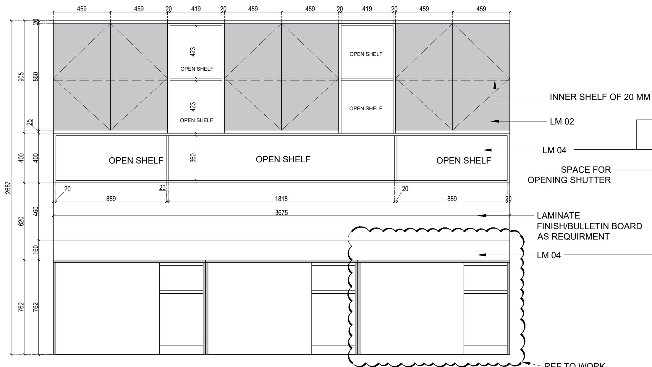
2 FRONT ELEVATION UPPERHEAD CABINATE
