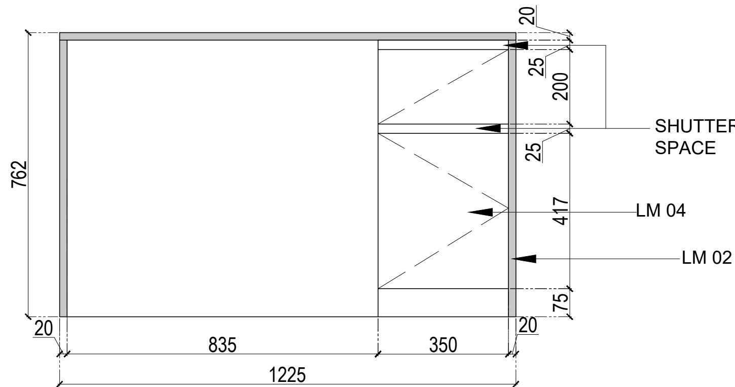
2 FRONT ELEVATION WORK STATION
