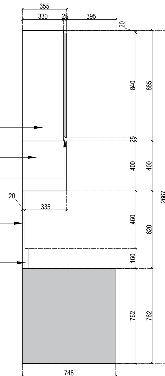
3 SIDE ELEVATION UPPERHEAD CABINATE
