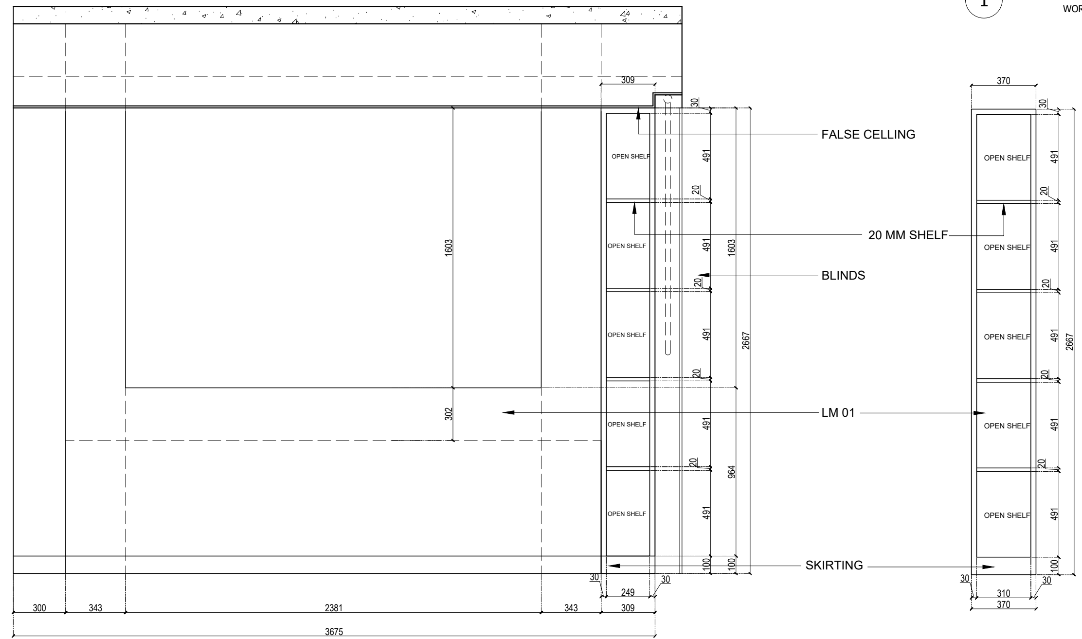
2.1 FRONT ELEVATION WORKSTATION AREA PLANTER BOX
