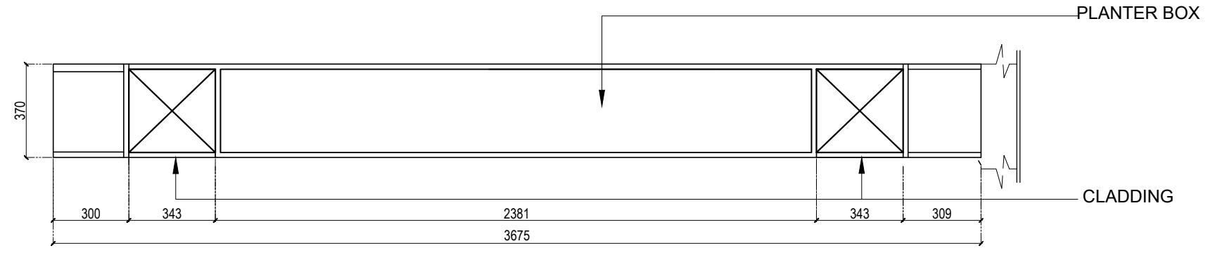
1 PLAN WORKSTATION AREA PLANTER BOX
