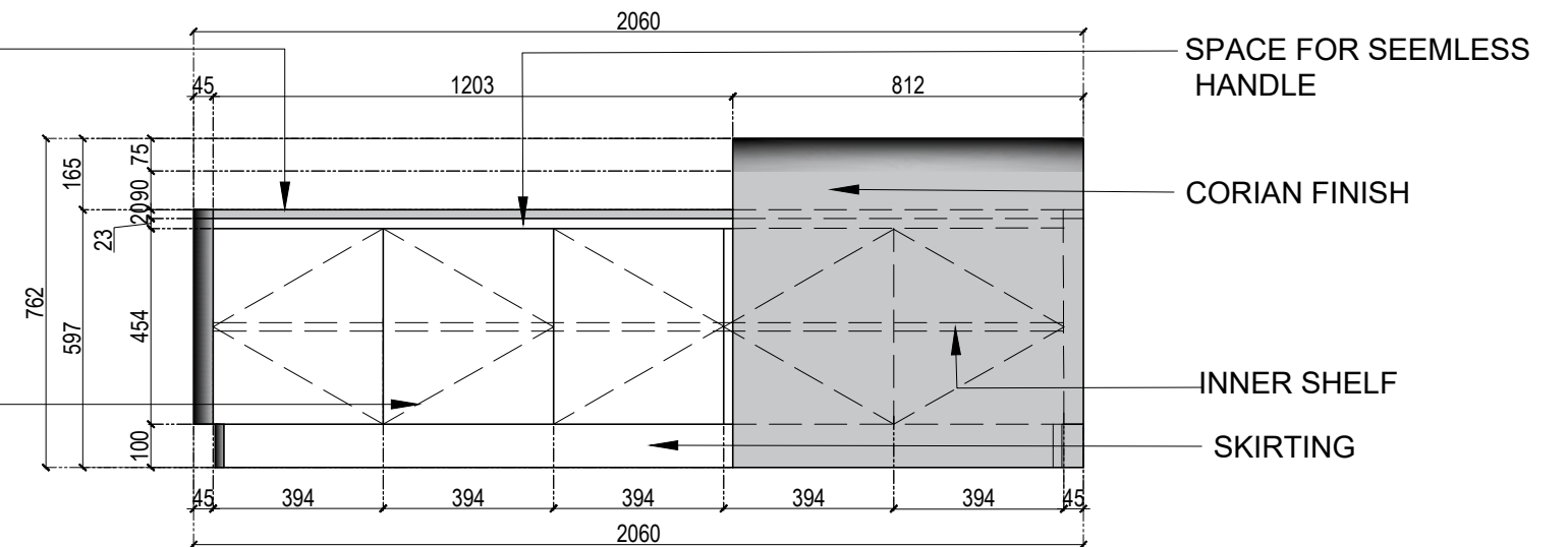
3 ELEVATION AT B DIRECTOR ROOM
