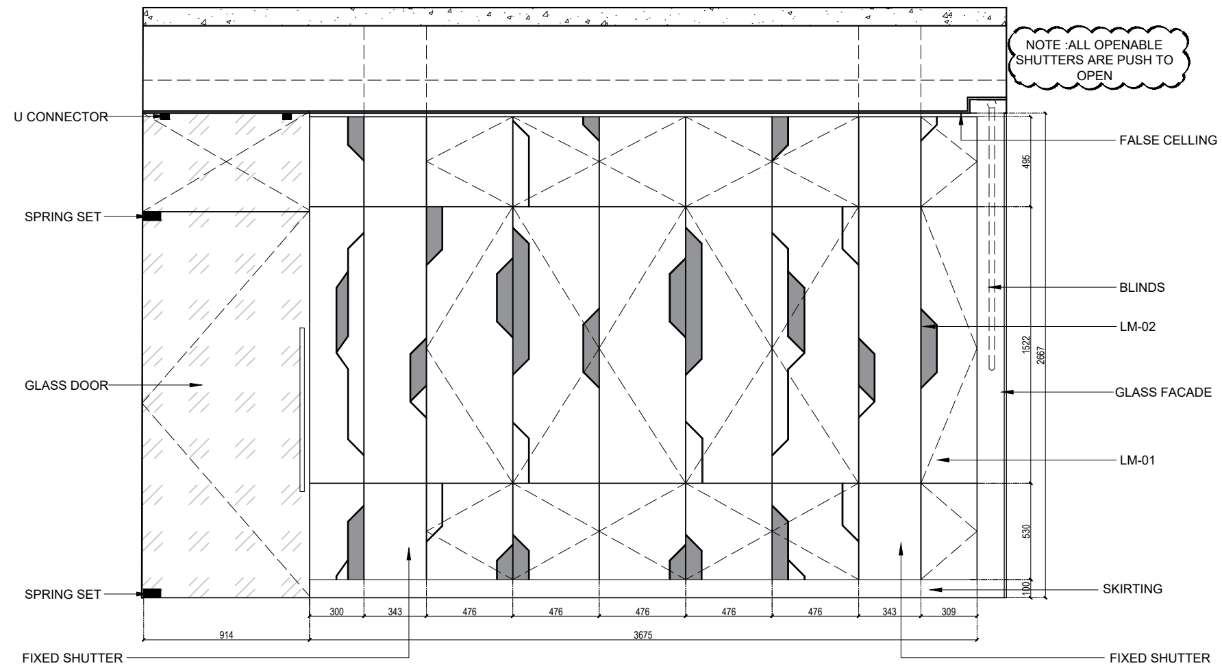
2.1 FRONT ELEVATION MD STORAGE CABINETE
