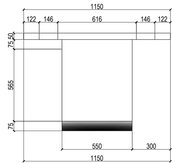
4 ELEVATION MEETING TABLE
